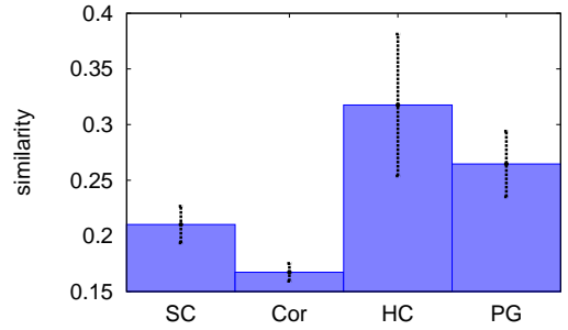
Fig. 4. Comparison of the different optimization methods. Hill climbing (HC) and policy gradient estimation (PG) perform significantly better than the single component (SC) and correlation-based (Cor) methods. All methods are able to greatly improve the similarity to the human gait. Shown are the mean and the 95% confidence interval.
